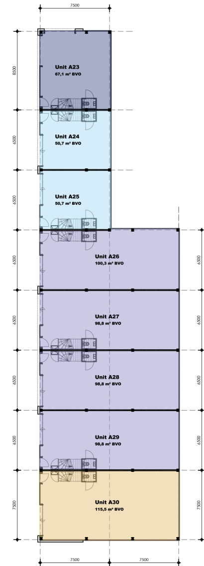
Begane grond Pand C Peil = 0 | 681 m² BVO
