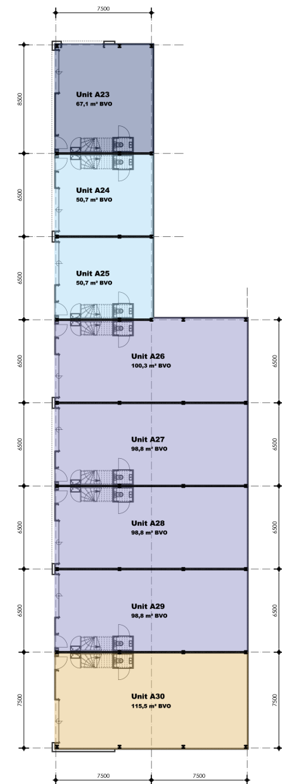
Begane grond Pand C Peil = 0 | 681 m² BVO
