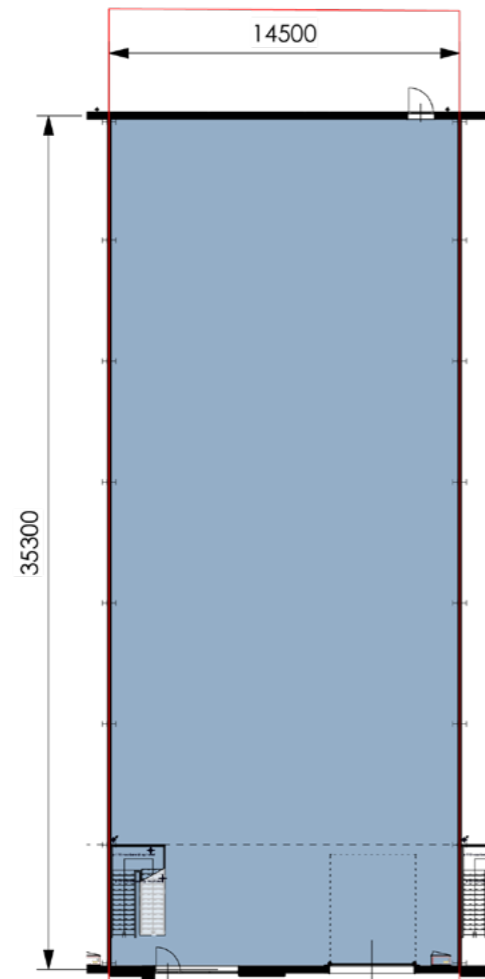
Begane grond - Unit 4 GO ±502 m 2
