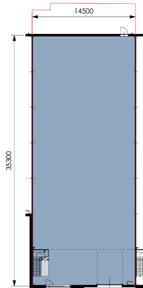
Begane grond - Unit 5 GO ±502 m 2
